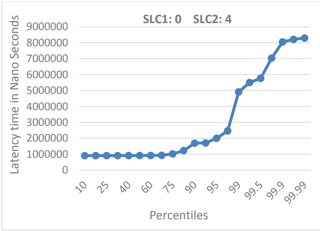
Fig. 18. RocksDB Read SLC factor variations for the data size : 100000 Bytes.
