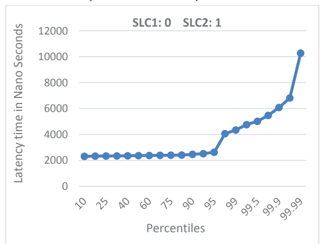
Fig. 13. RocksDB Write SLC factor variations for the data size : 100 Bytes
